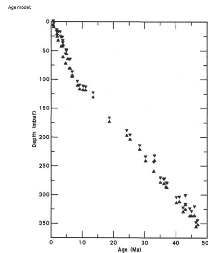
Figure 17. Age-depth plot showing sedimentation rates at Site 709.
