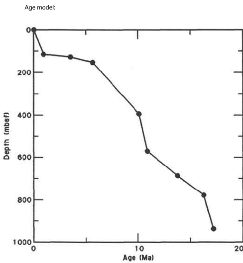
Figure 8. Sediment accumulation rate at Site 718.
