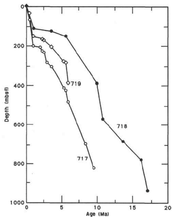
Figure 8. Sediment accumulation rates at Sites 717, 718, and 719.
