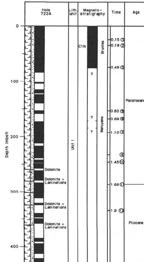
Magnetostratigraphy
