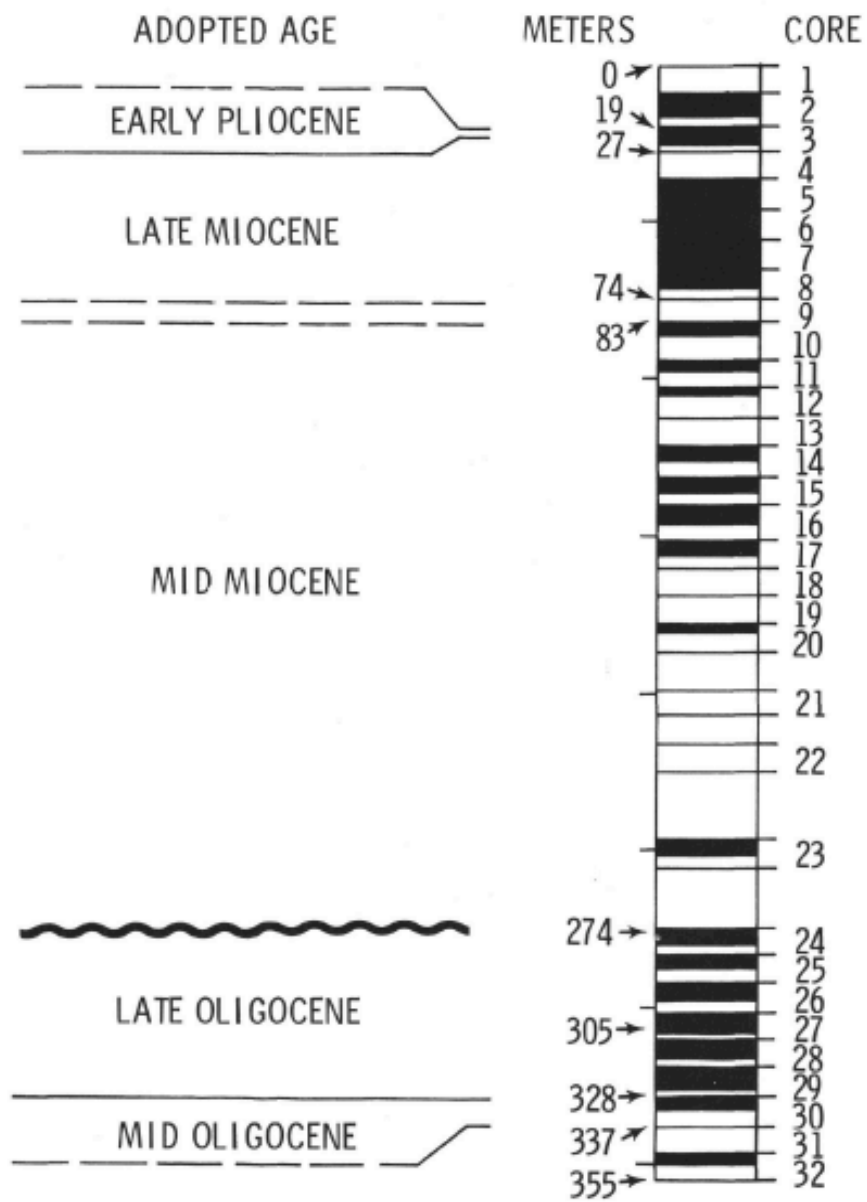
Figure 4. Biostratigraphy of Site 205 as deduced from the calcareous nannofossils.
