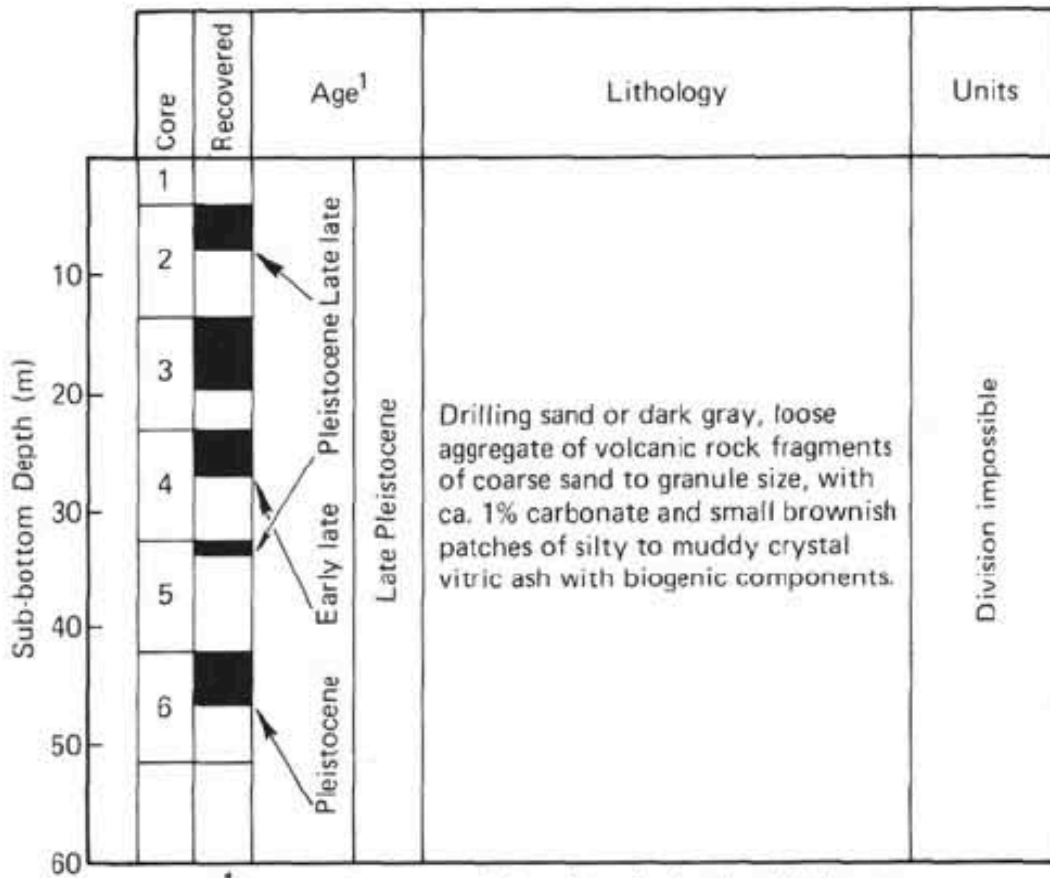
1 Arrows show sample locations for late late Pleistocene and early late Pleistocene determinations.
