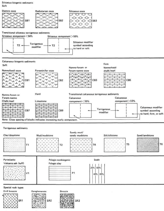
Figure 4. Symbols used in graphic lithology columns of core description forms (sediment).
