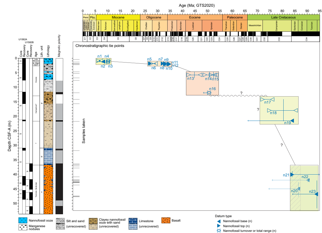
Figure F21. Age-depth model primarily based on calcareous nannofossil biostratigraphy and magnetostratigraphy, Site U1582. Numbers for bioevents correspond to those in Table T4. GTS2020 = Geologic Time Scale 2020 (Gradstein et al., 2020). Colored boxes = approximate ages of sediment packages based on inferred in situ nannofossil assemblages; background color correlates to the geologic timescale. Events n21 and n22 are tentative because they are based on single specimens in only a few samples. Black undulating line = unconformity.
